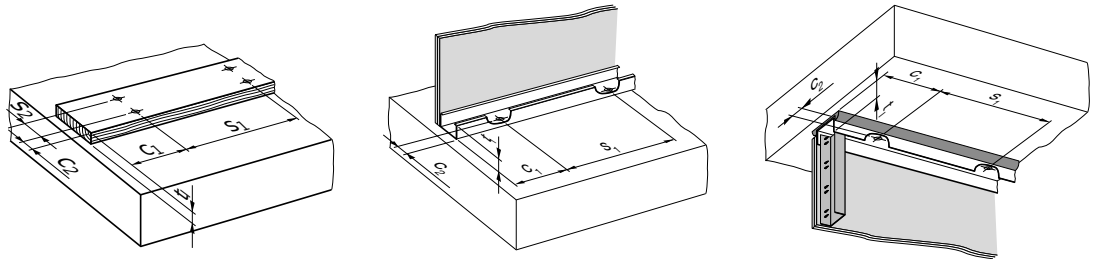
Deflection head track fastening (optional with sealant)
