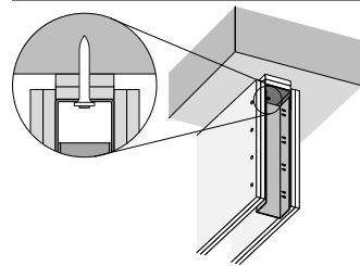
Deflection head fastening with gypsum strips (optional with sealant)
