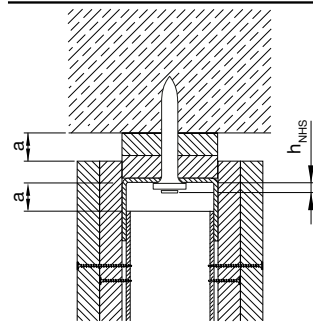
Deflection head fastening with gypsum strips (optional with sealant)
