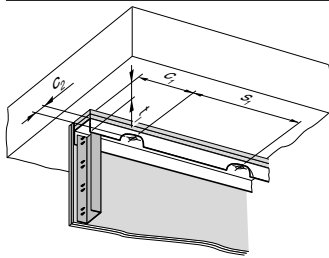
Deflection head fastening with gypsum strips (optional with sealant)
